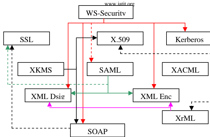
Figure 1: This model has been chosen to facilitate combining of end-point, the following consequences flow from the model. The first we can show WS-Security is Refer to Composite standard, the WS-Security defines a set of SOAP header extensions for end-to-end SOAP messaging security. It supports message integrity and confidentiality by allowing communicating partners to exchange signed encrypted messages in a Web services environment, XKMS is the Public-key infrastructure -An XML protocol that allows a simple client to obtain key information (value, certificate, management, or trust data) from a Web service. It also describes protocols for distributing and registering public keys, suitable for use in conjunction with the standards for XML Signature and XML encryption. XrML and XACML Access control of the process which Appearing in the plan. The Task of the Technologies for securing representation on the SAML, Kerberos and X.509 is Security tokens (authentication assertions). Assignment of the XML Enc, XML Dsig and SSL is Confidentiality and integrity information, finally the SOAP Working Role is transport message. The Details of the process we have already discussed in the body of the paper.
