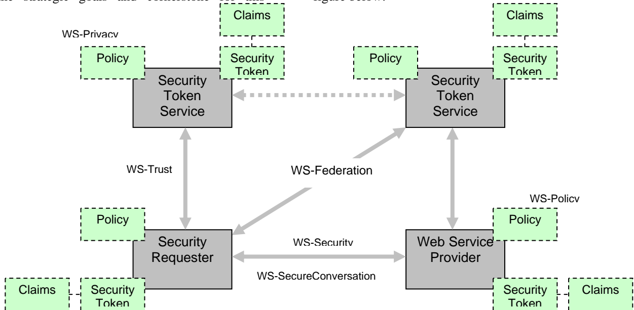
Figure2: Web Services Security Stages
