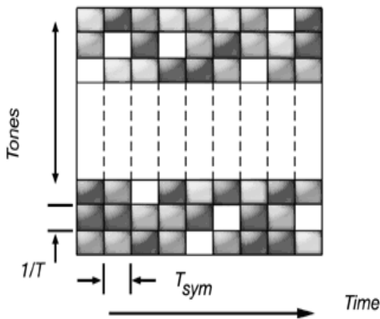
Figure 3. Two-Dimensional Illustration of OFDM Channel Resource
