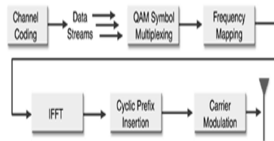
Figure 2. OFDM Transmitter Chain
