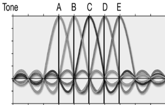
Figure 1. OFDM Tones
