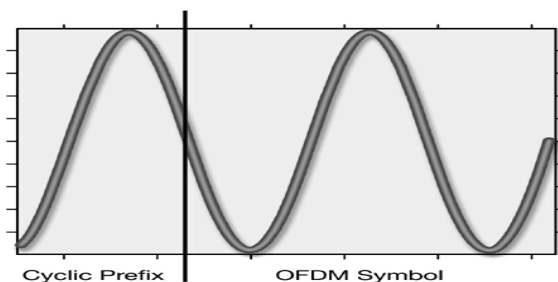
Figure 6. Cyclic Extension of Sinusoid
