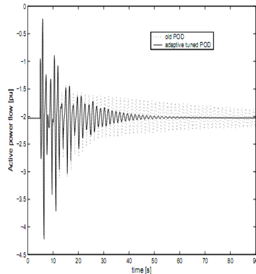
Fig. 10. Active power flow in the controlled line 34-37 after three phase fault applied to line 33-34 and with lines 31-32 and 12-26 out of service.
