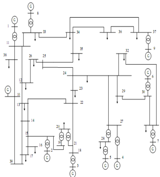
Fig. 2. System configuration for the case study
