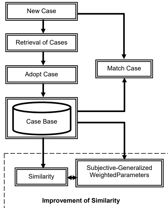
Figure 1: Proposed Model for Improvement of CBR
