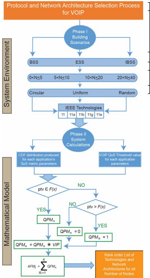
Figure 1: Flowchart of the proposed algorithm
