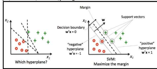
Figure 1. Support vector machine
