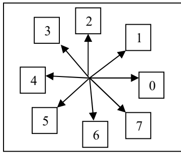
Figure2: 8-connected neighbors
