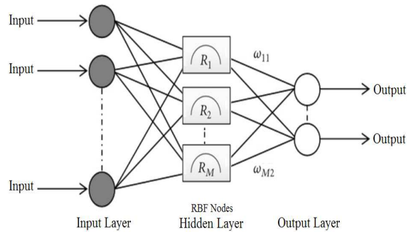
Figure 5: RBF-NN Basic Structure
