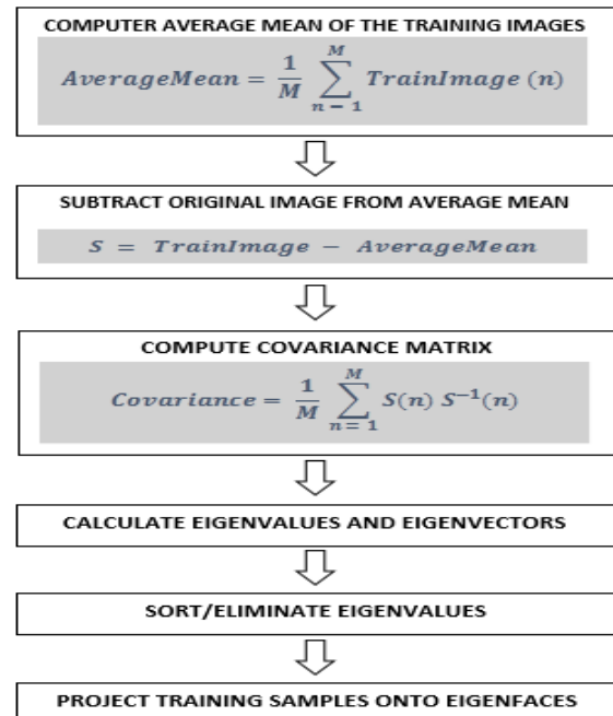
Figure 3: PCA Block Diagram
