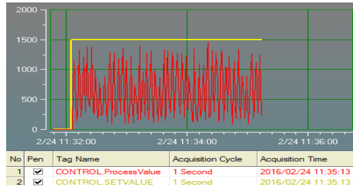
Figure 21. Graphic KP=KI=KD=100
