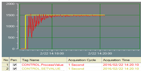
Figure 10. Graphic KP = KI = 100
