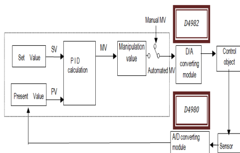
Figure 6: System Control Close Loop
