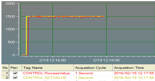
Figure 15. Graphic KP=KI=KD=1
