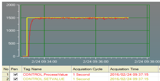
Figure 9. Graphic KP = KI = 10
