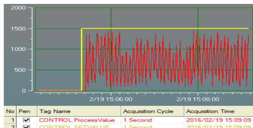
Figure 18. Graphic KP=1 KI=1 KD=100
