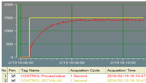
Figure 17. Graphic KP=1 KI=100 KD=1
