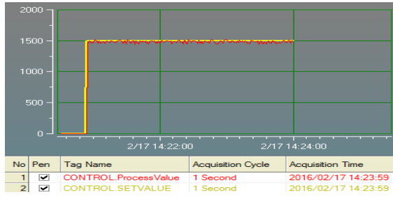
Figure 8. Graphic KP = KI = 1
