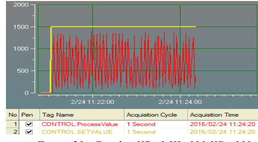
Figure 20. Graphic KP=1 KI=100 KD=100
