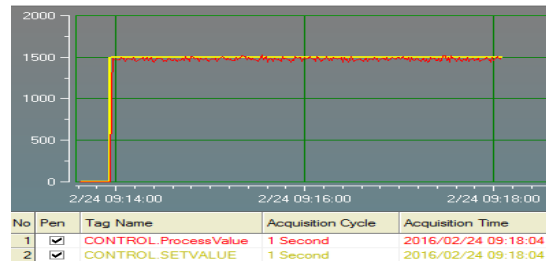
Figure 13. Graphic KP=10 , KI=1
