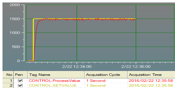
Figure 11. Graphic KP=1 KI=10
