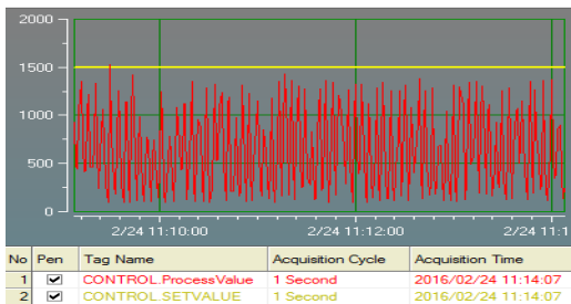
Figure 19. Graphic KP=100 KI=1 KD=100
