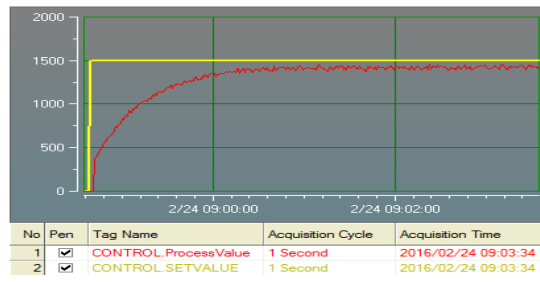
Figure 12. Graphic KP=10 KI=100
