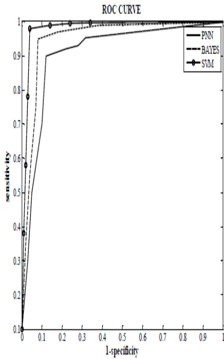
Fig 17 ROC Curve for Comparison of PNN Bayes and SVM
