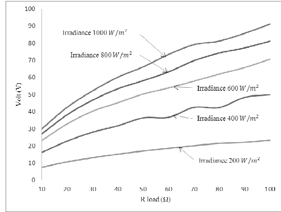
Figure 16: Curve of Comparison Load Voltage With Load Resistance at MPPT Method
