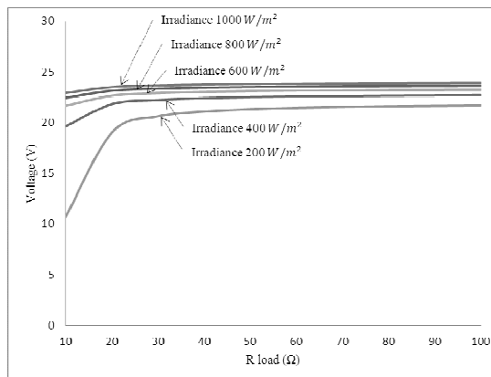
Figure 13: Curve of Comparison Load Voltage With Load Resistance at Direct-Coupled Method
