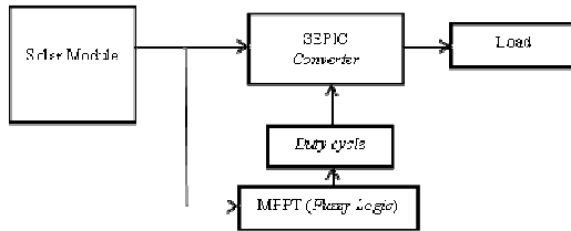
Figure 2: Diagram Block
