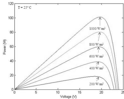
Figure 10: Curve Characteristic of V-P
