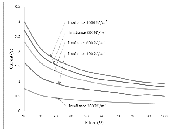
Figure 17: Curve of Comparison Load Current With Load Resistance at MPPT Method
