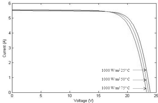
Figure 7: Temp Influence to V-I Curve
