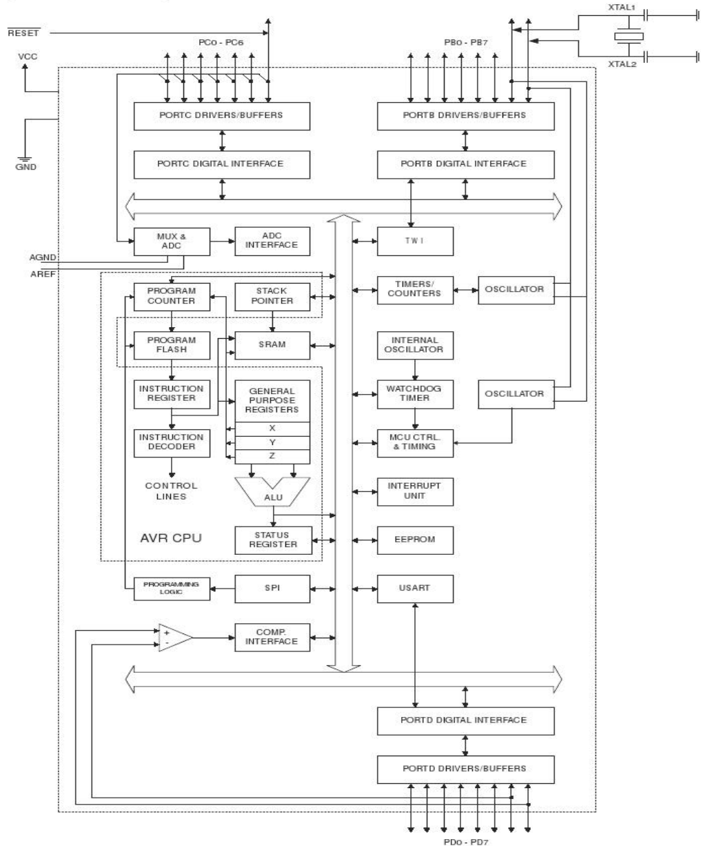
Figure 2. Block Diagram Of Atmega8 Microcontroller
