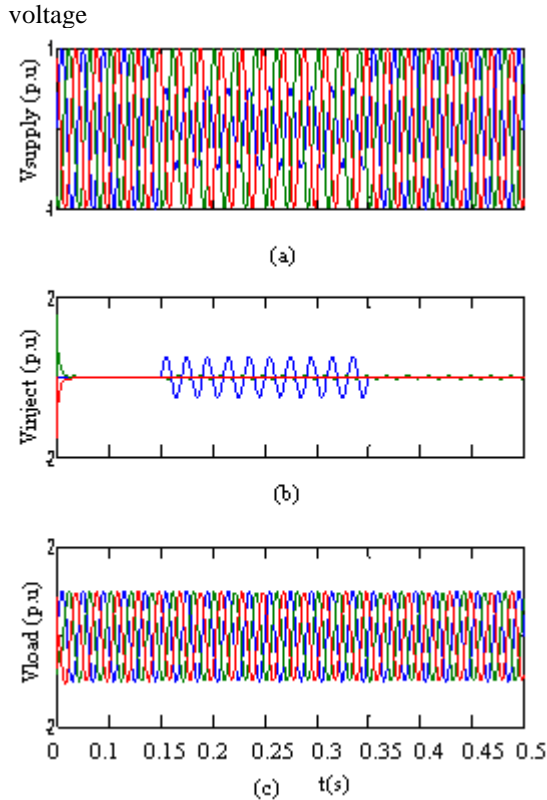
Figure 6 Single-phase voltage sag: (a)-Source voltage, (b)-Injected voltage, (c)-Load voltage
