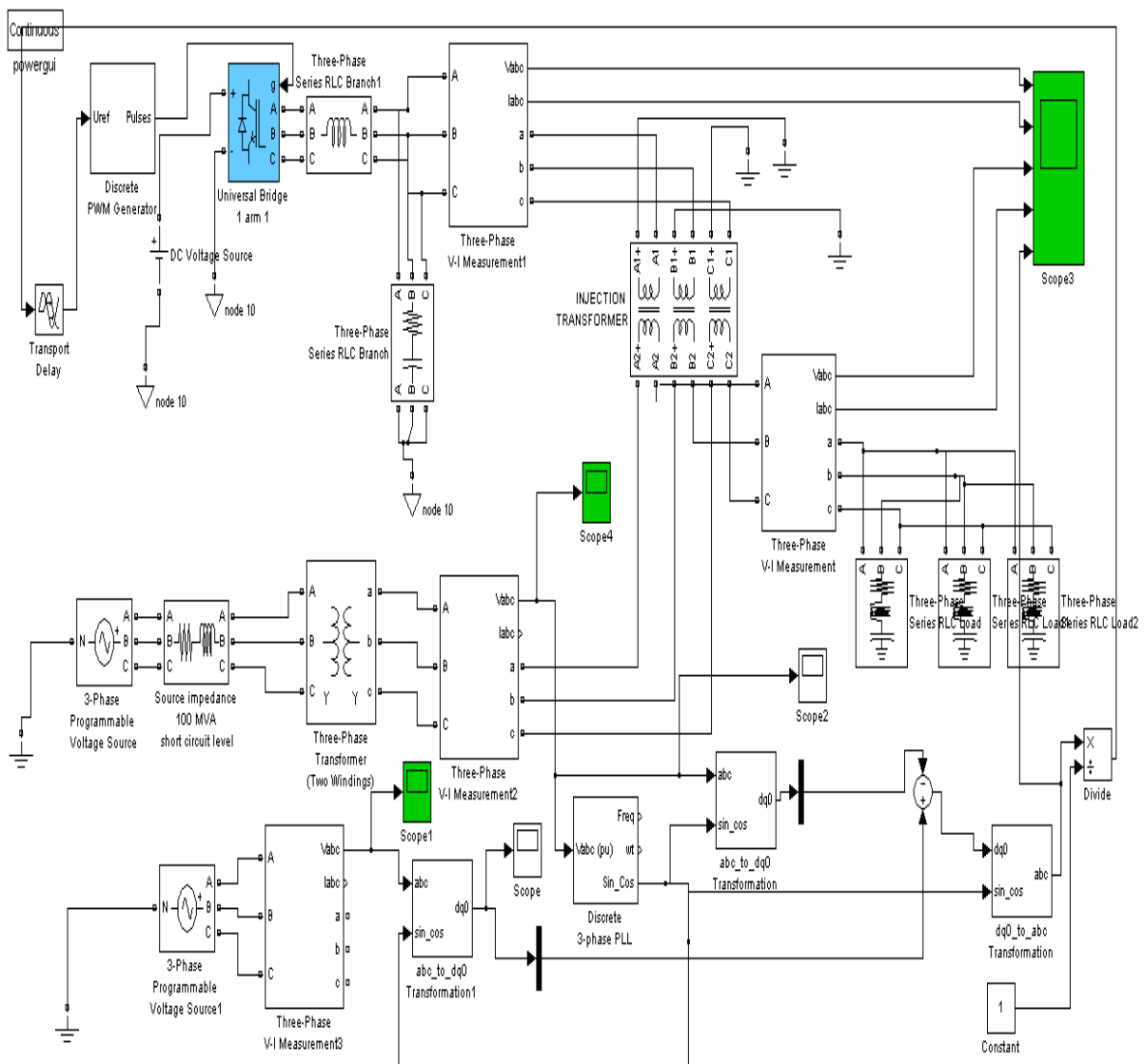
Figure 3: Proposed system configuration
