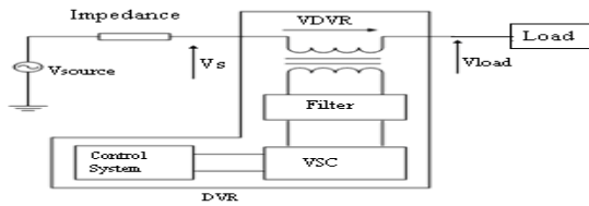
Figure 1: Schematic diagram of DVR
