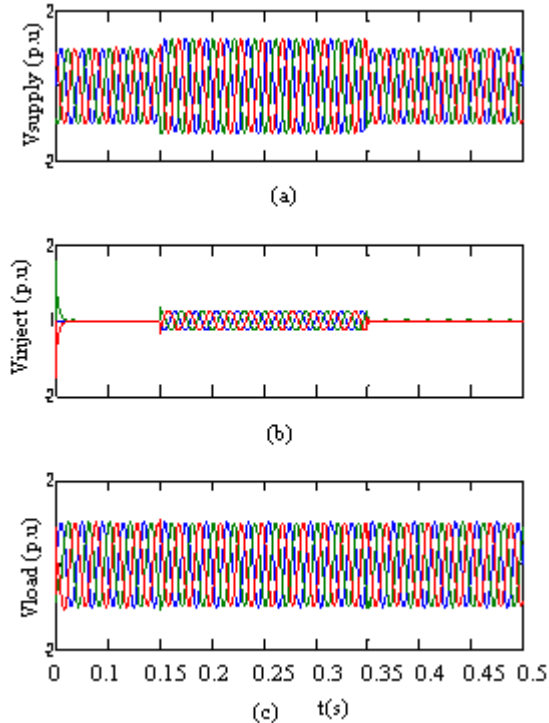
Figure 7 Three-phase voltages swell: (a)-Source voltage, (b)-Injected voltage, (c)-Load voltage
