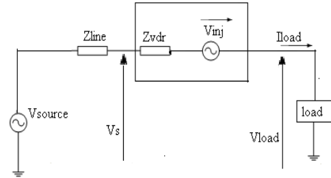
Figure 2: Equivalent Circuit of DVR
