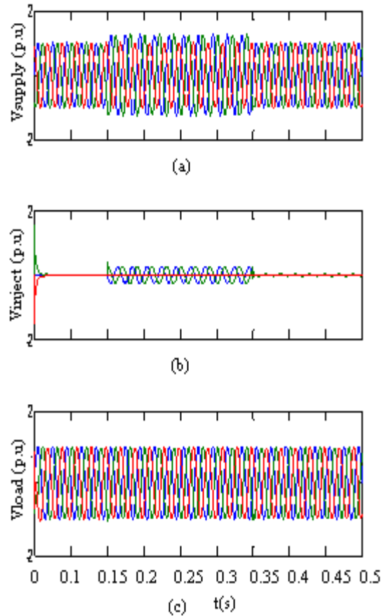
Figure 8 Two-phase voltages swell: (a)-Source voltage, (b)-Injected voltage, (c)-Load voltage
