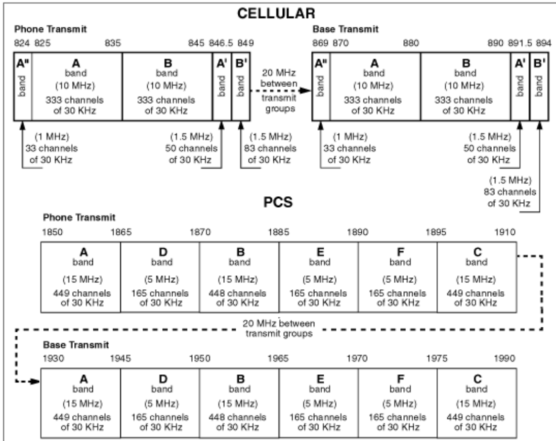
Figure 3. Comparison of Cellular and PCS Spectrums
