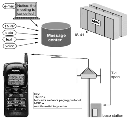
Figure 1. PCS Teleservice Messaging Scheme
