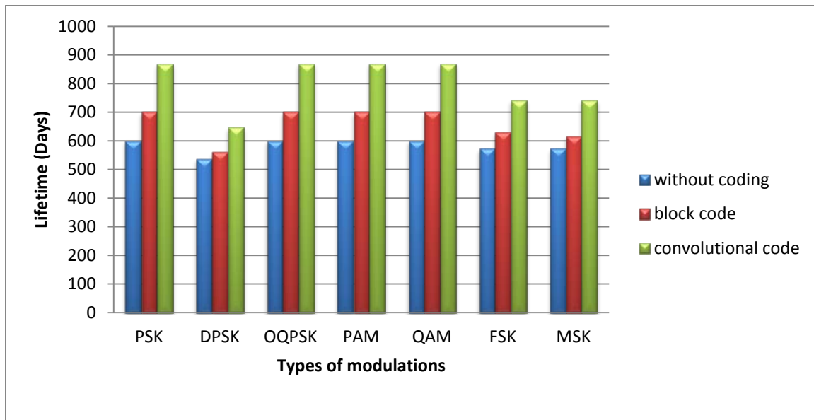
Figure 9: Lifetime Of WSN For Different Modulation And Coding At D=5m
