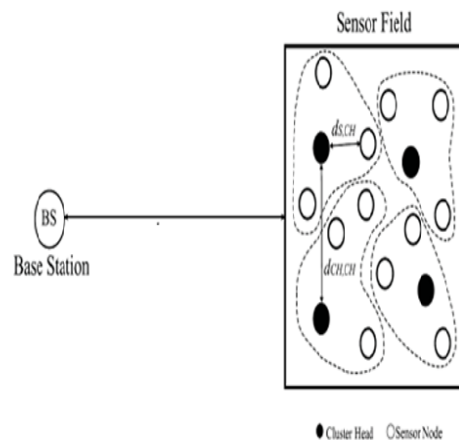
Figure 1 : WSN model
