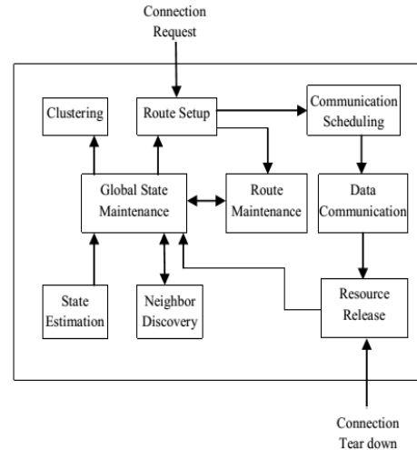
Figure 2: QoS Enhanced Base Station Controlled Dynamic Clustering Protocol
