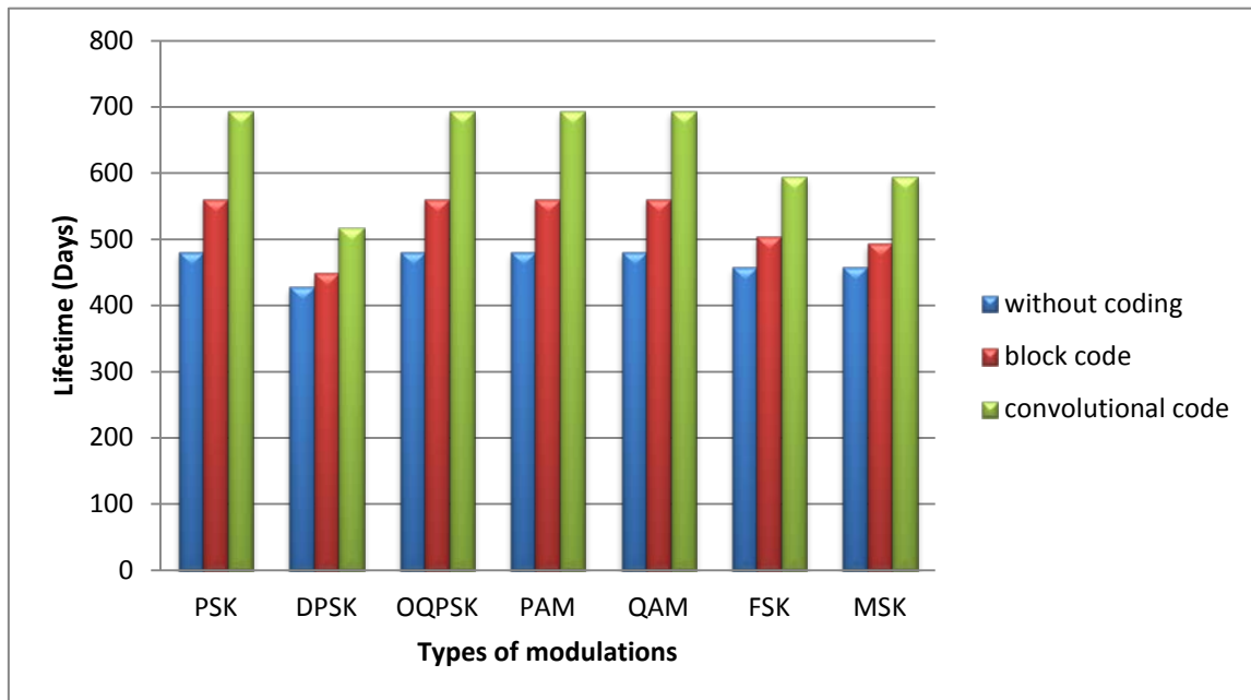
Figure 9: Lifetime Of WSN For Different Modulation And Coding At D=5m
