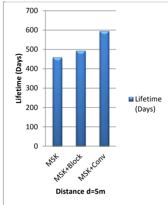
Figure 5: Comparison Of MSK Modulation With & Without Coding At Distance D=5m
