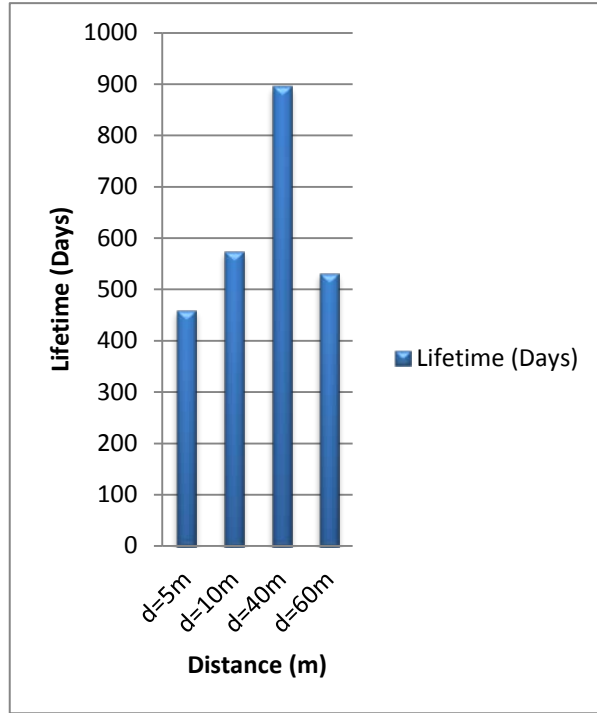
Figure 4: Distance Vs Lifetime for MSK without coding
