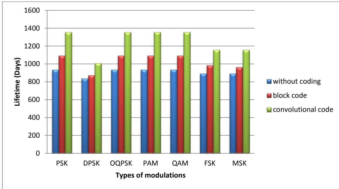
Figure 11: Lifetime Of WSN For Different Modulation And Coding At D=40m
