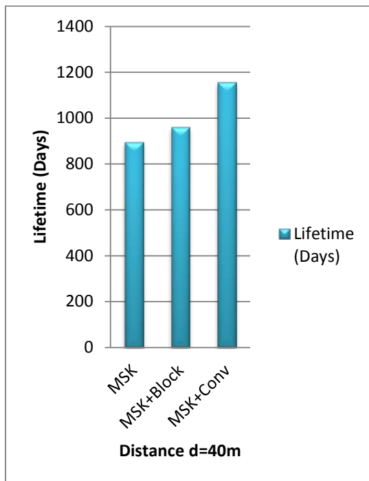
Figure 7: Comparison Of MSK Modulation With & Without Coding At Distance D=40m
