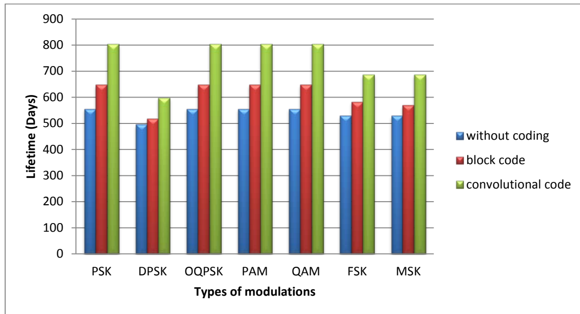
Figure 12: Lifetime Of WSN For Different Modulation And Coding At D=60m
