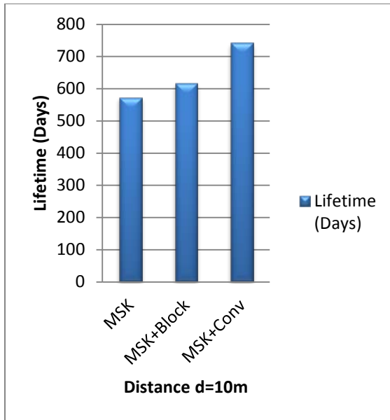
Figure 6: Comparison Of MSK Modulation With & Without Coding At Distance D=10m
