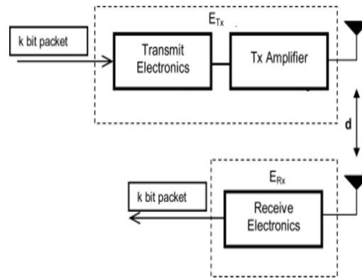
Figure 3: Sensor Node Energy Model
