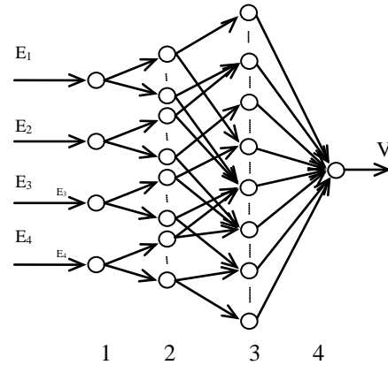
Figure 2: FNN Neural Network
