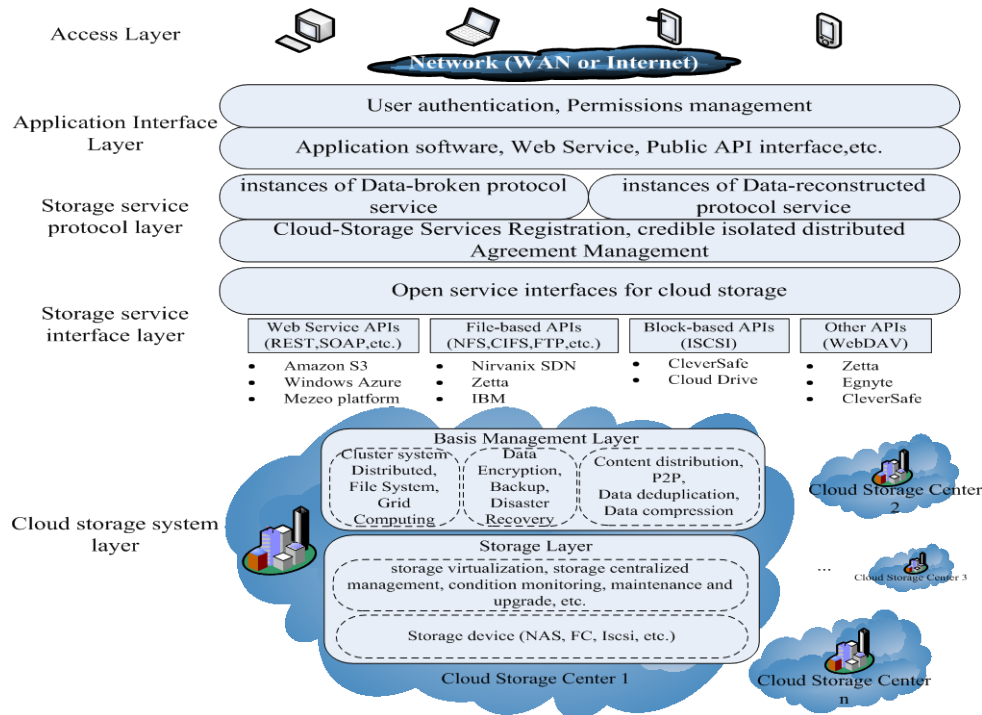
Figure 1. Isolated Distributed Services Architecture Based On Structured Strategy.
