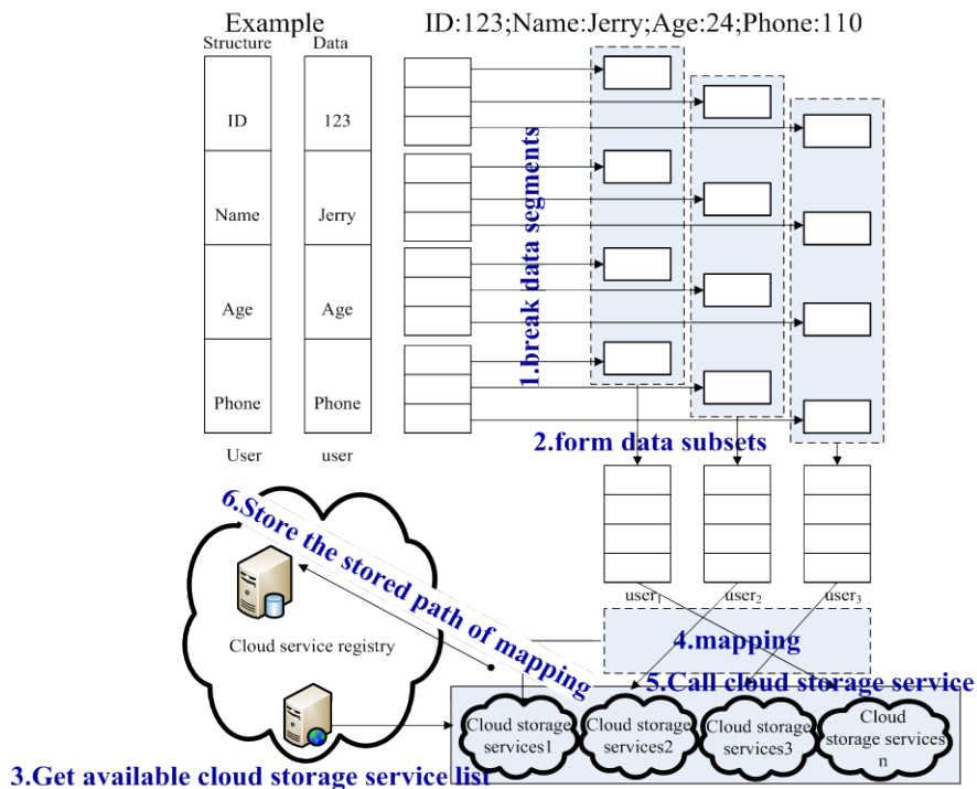
Figure 2. The Basic Process For Structured Isolated Distributed Storage.
