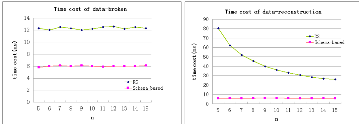
Figure 3. Time Cost Of Data-Broken And Data-Reconstruction.
