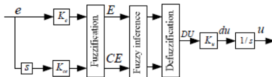
Fig. 1. Block of FLC
